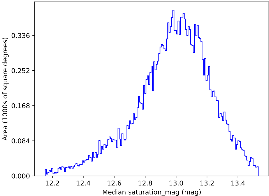
too_100_4v3.4_10yrs All sky u band: Median saturation_mag
