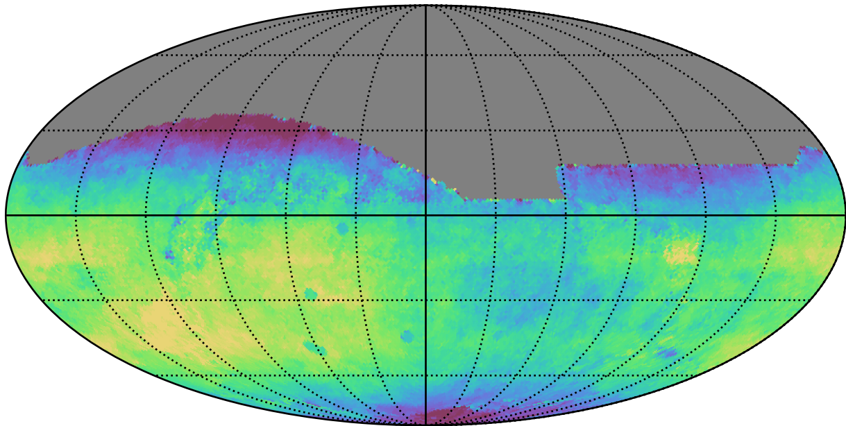
too_100_4v3.4_10yrs All sky r band: Median saturation_mag
