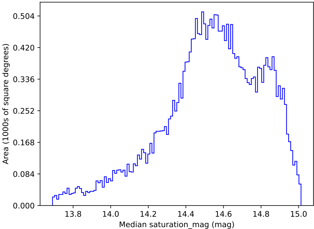
too_100_4v3.4_10yrs All sky r band: Median saturation_mag
