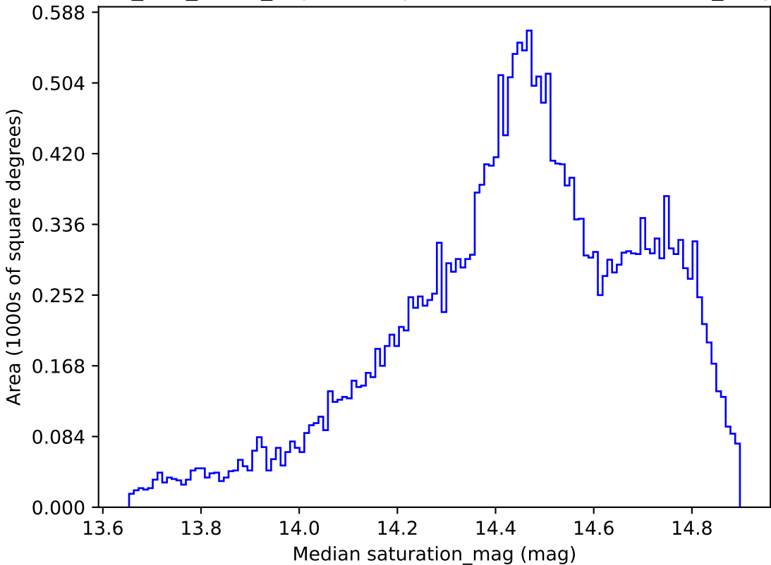
too_100_4v3.4_10yrs All sky i band: Median saturation_mag
