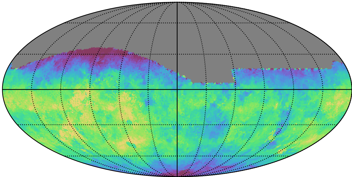
too_100_4v3.4_10yrs All sky g band: Median saturation_mag
