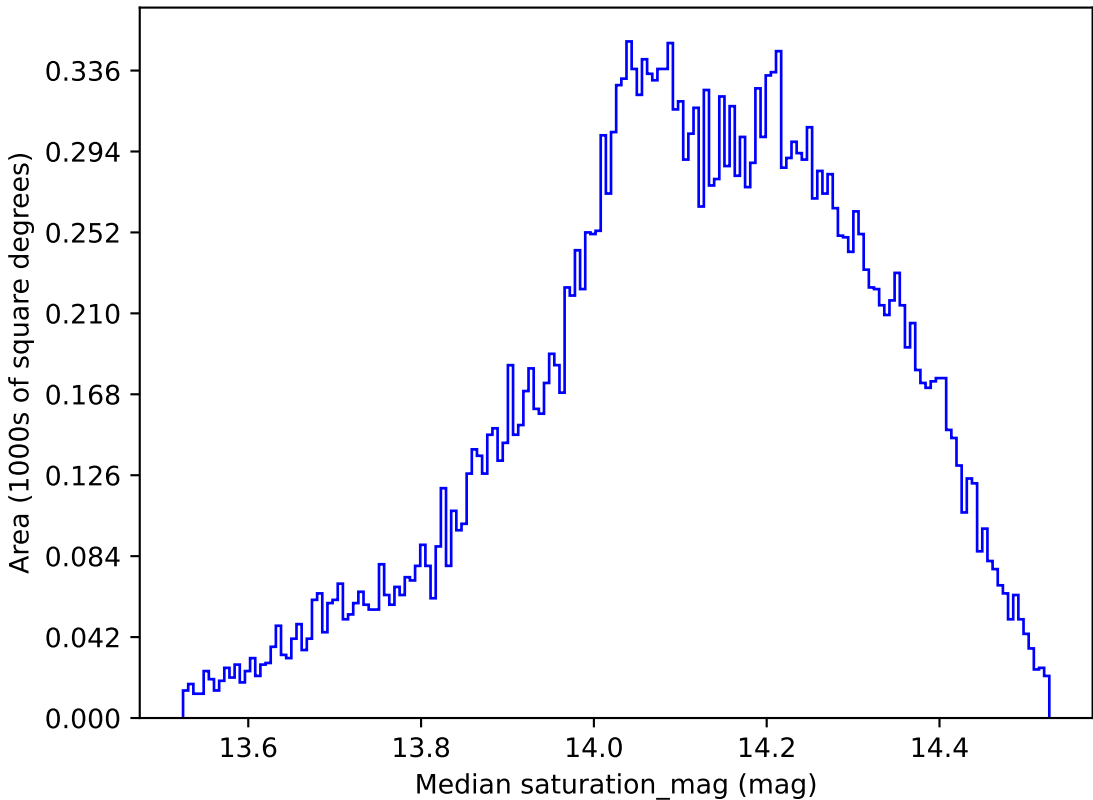
too_100_4v3.4_10yrs All sky all bands: Median saturation_mag
