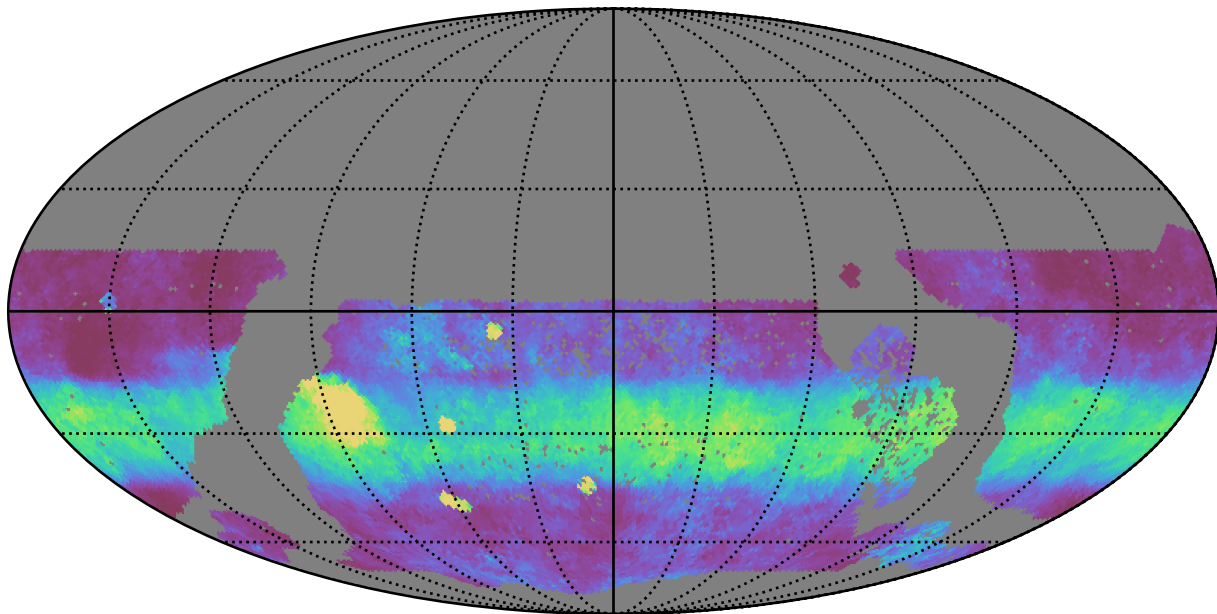
too_100_4v3.4_10yrs WFD z band: Median normairmass
