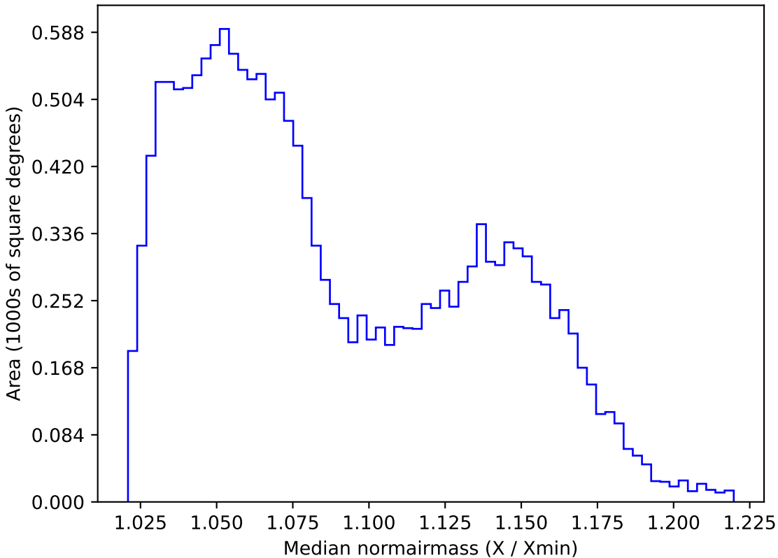
too_100_4v3.4_10yrs WFD z band: Median normairmass
