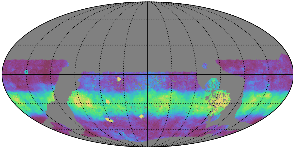
too_100_4v3.4_10yrs WFD y band: Median normairmass
