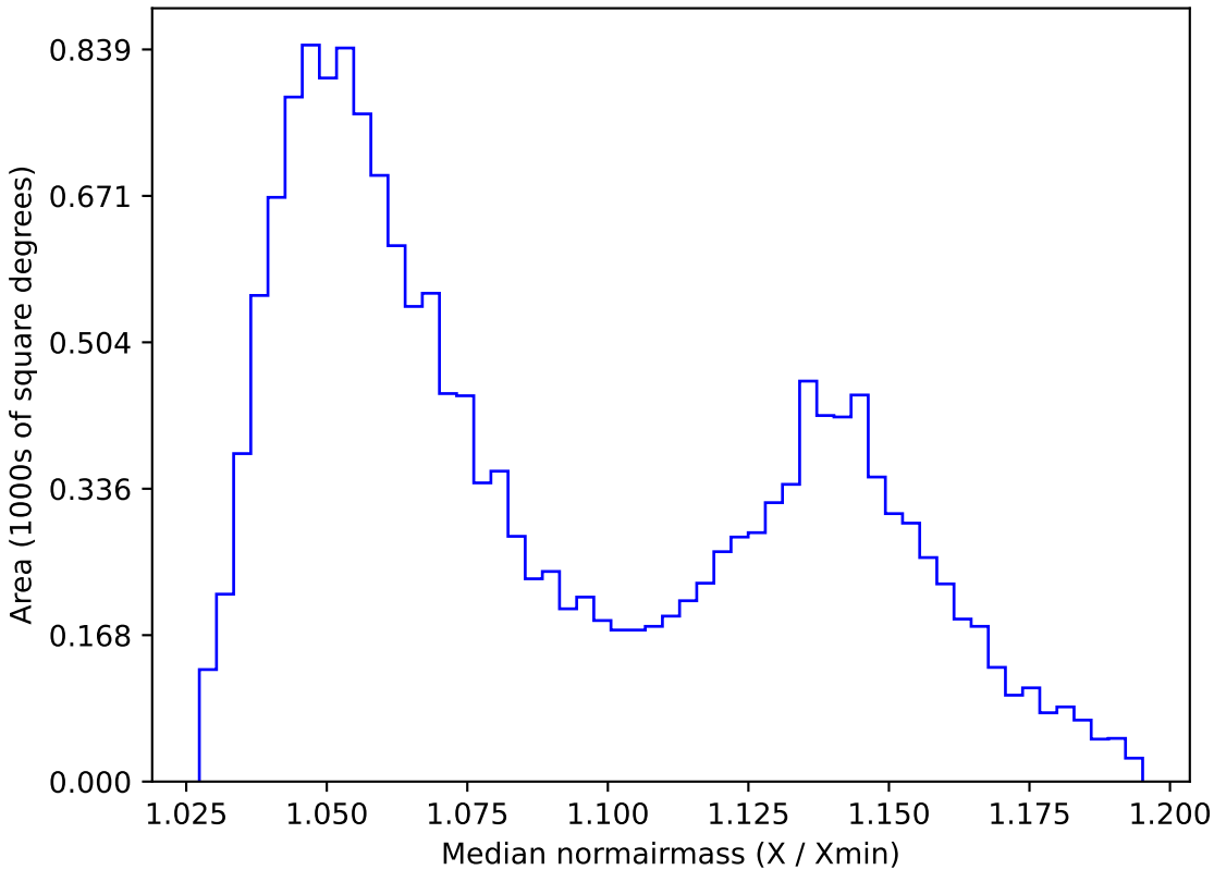
too_100_4v3.4_10yrs WFD y band: Median normairmass
