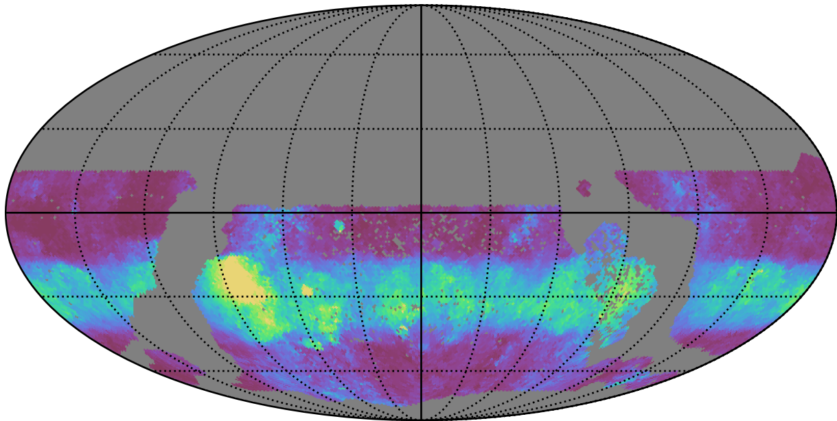
too_100_4v3.4_10yrs WFD u band: Median normairmass
