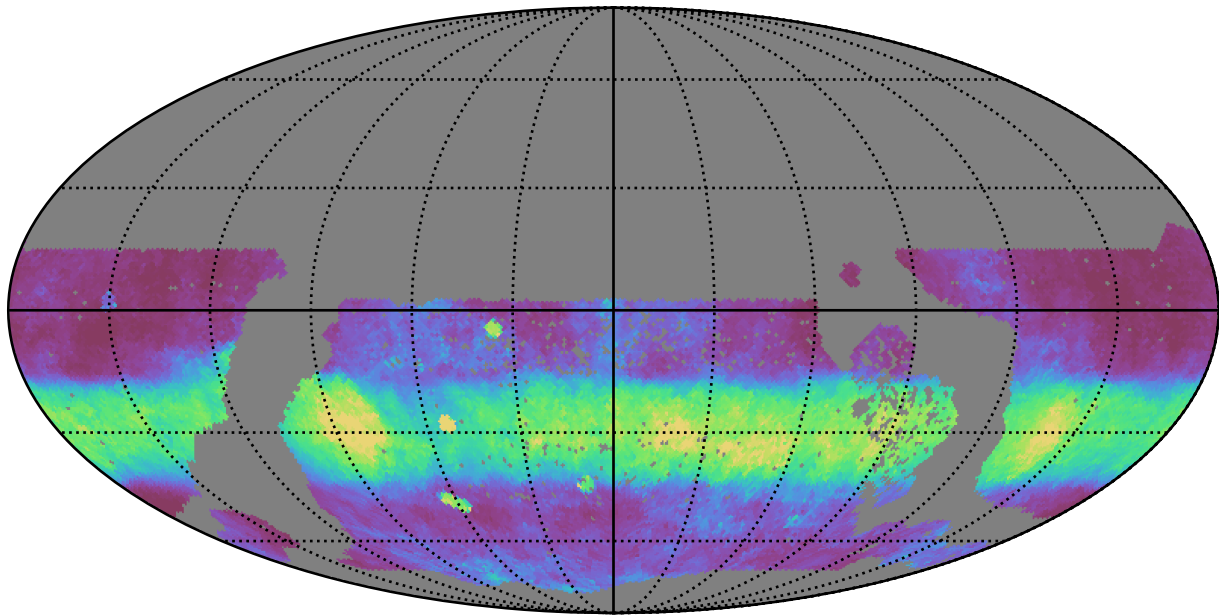
too_100_4v3.4_10yrs WFD i band: Median normairmass
