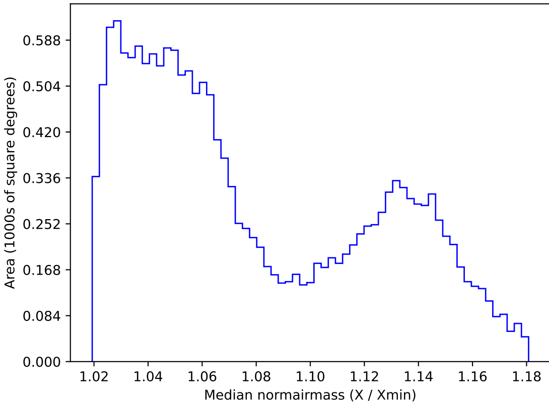
too_100_4v3.4_10yrs WFD i band: Median normairmass
