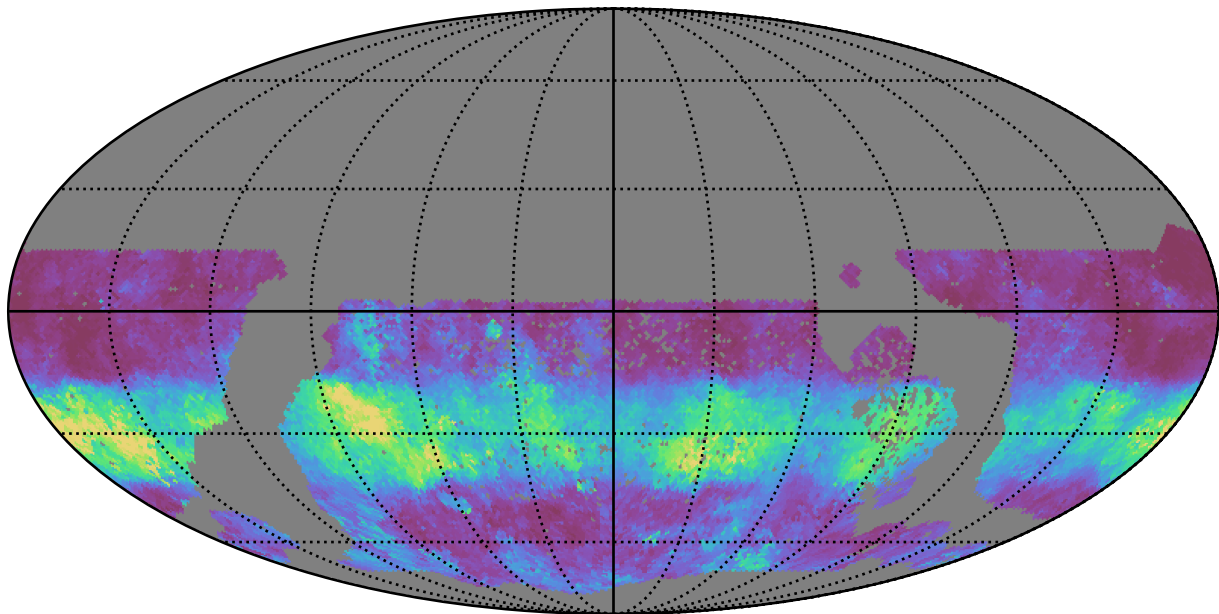
too_100_4v3.4_10yrs WFD g band: Median normairmass
