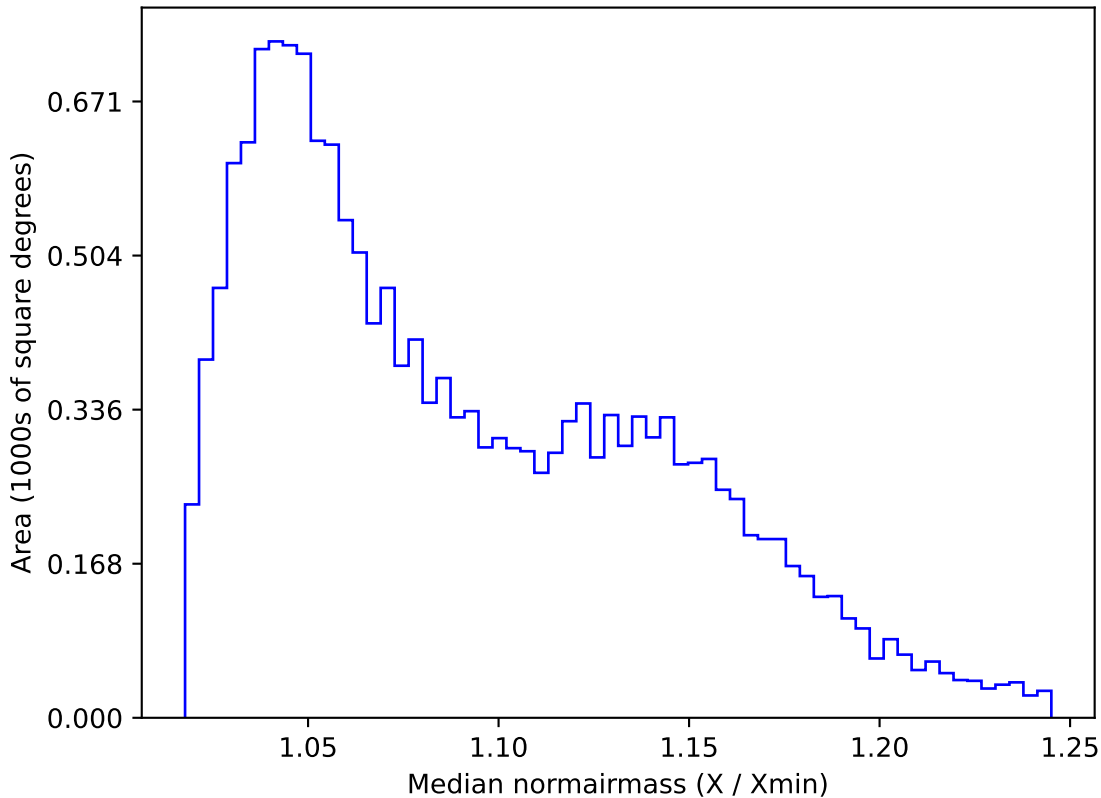
too_100_4v3.4_10yrs WFD g band: Median normairmass
