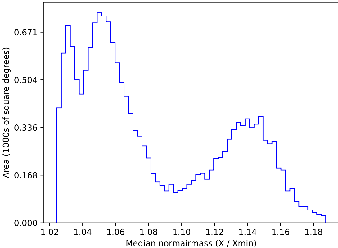
too_100_4v3.4_10yrs WFD all bands: Median normairmass
