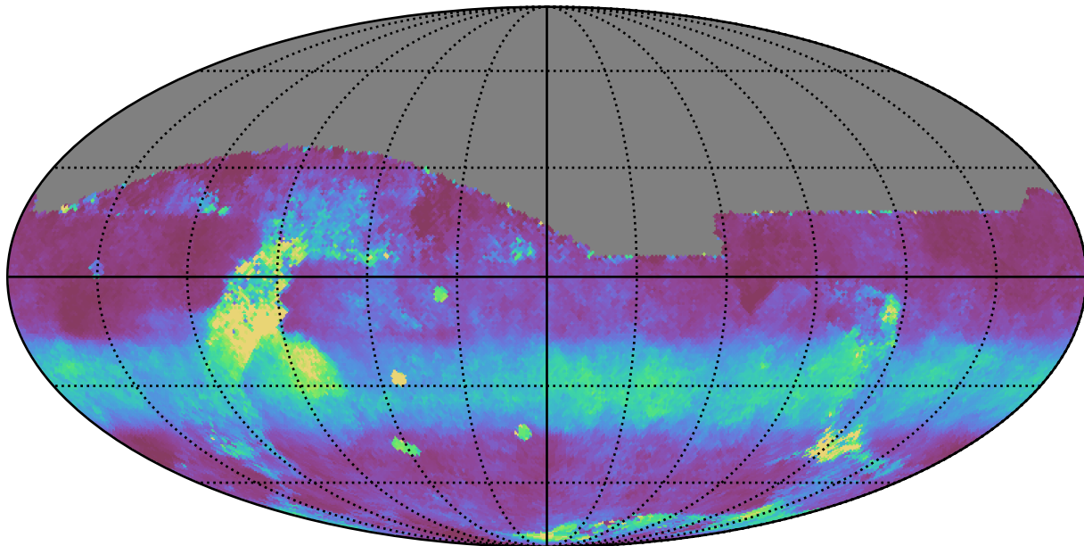
too_100_4v3.4_10yrs All sky z band: Median normairmass
