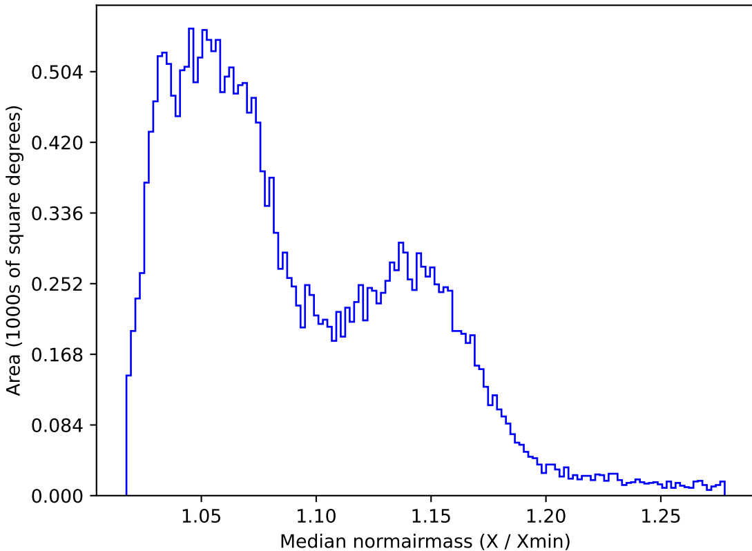
too_100_4v3.4_10yrs All sky z band: Median normairmass
