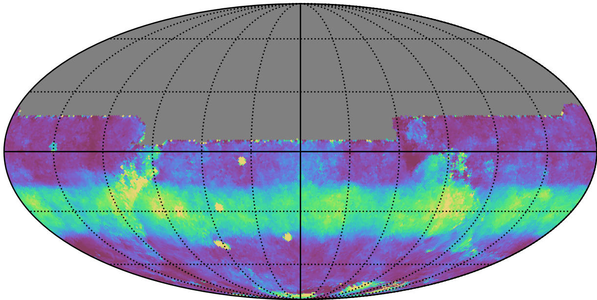
too_100_4v3.4_10yrs All sky y band: Median normairmass
