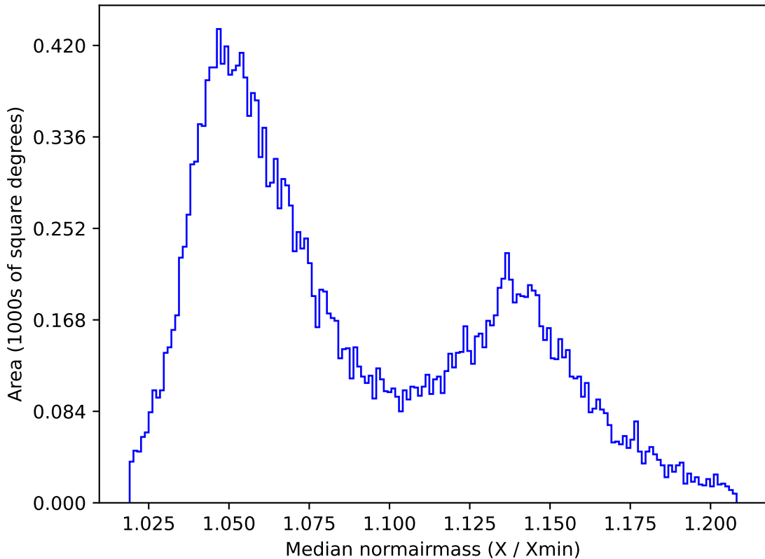
too_100_4v3.4_10yrs All sky y band: Median normairmass
