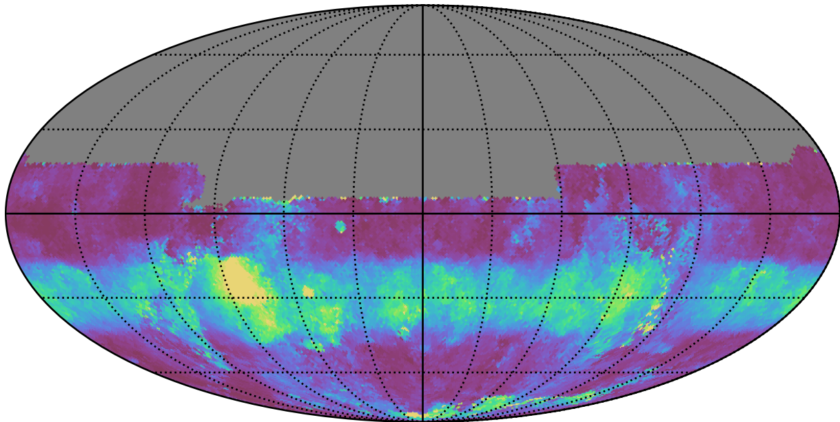
too_100_4v3.4_10yrs All sky u band: Median normairmass
