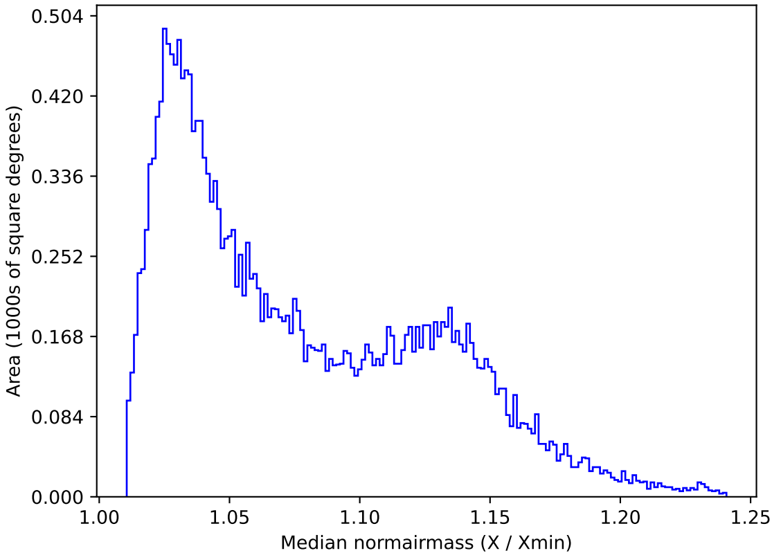
too_100_4v3.4_10yrs All sky u band: Median normairmass
