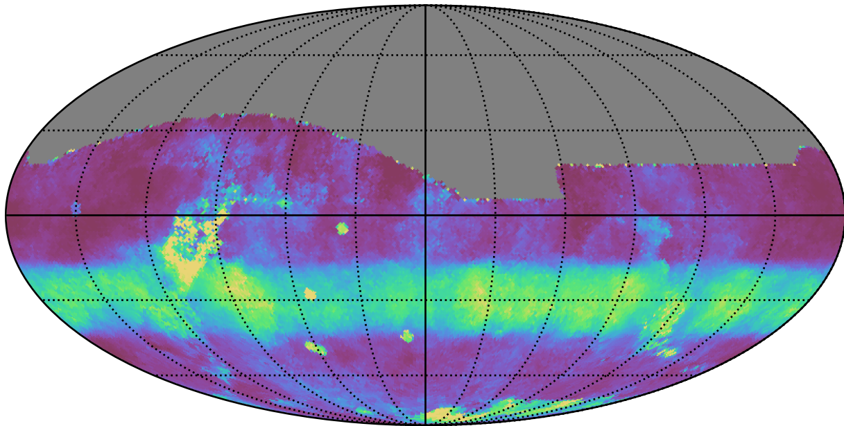
too_100_4v3.4_10yrs All sky r band: Median normairmass
