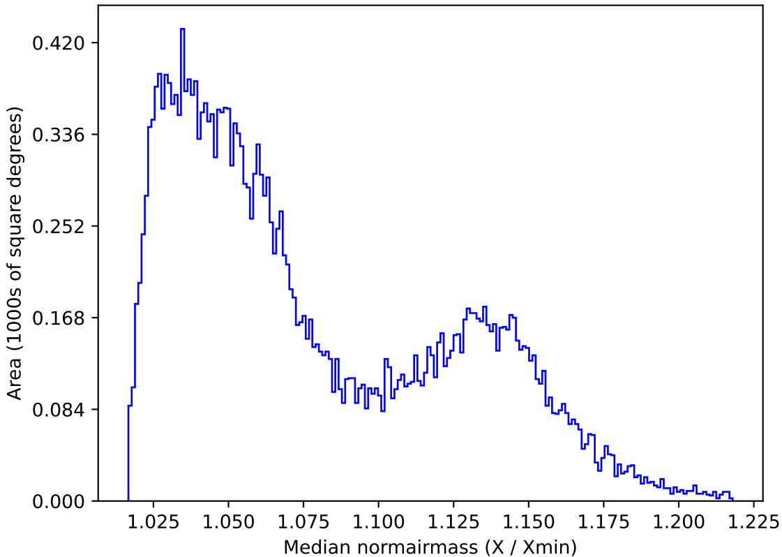
too_100_4v3.4_10yrs All sky i band: Median normairmass
