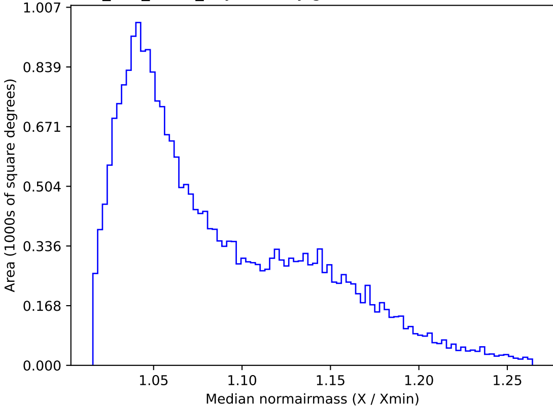
too_100_4v3.4_10yrs All sky g band: Median normairmass
