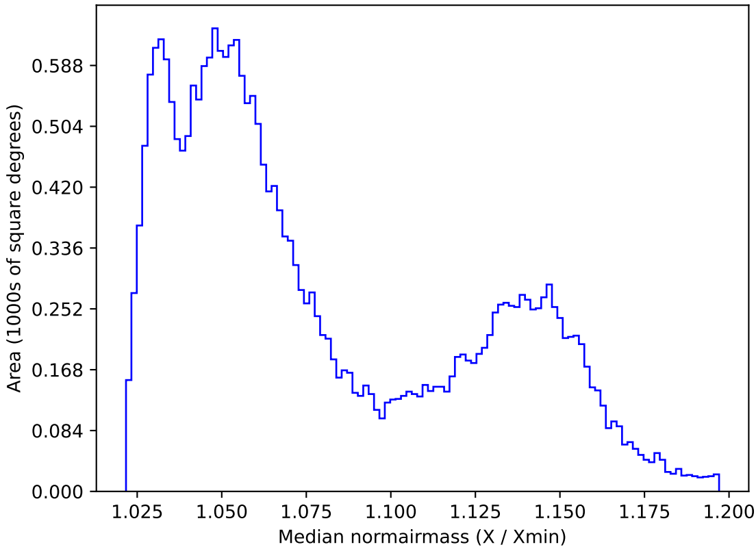
too_100_4v3.4_10yrs All sky all bands: Median normairmass
