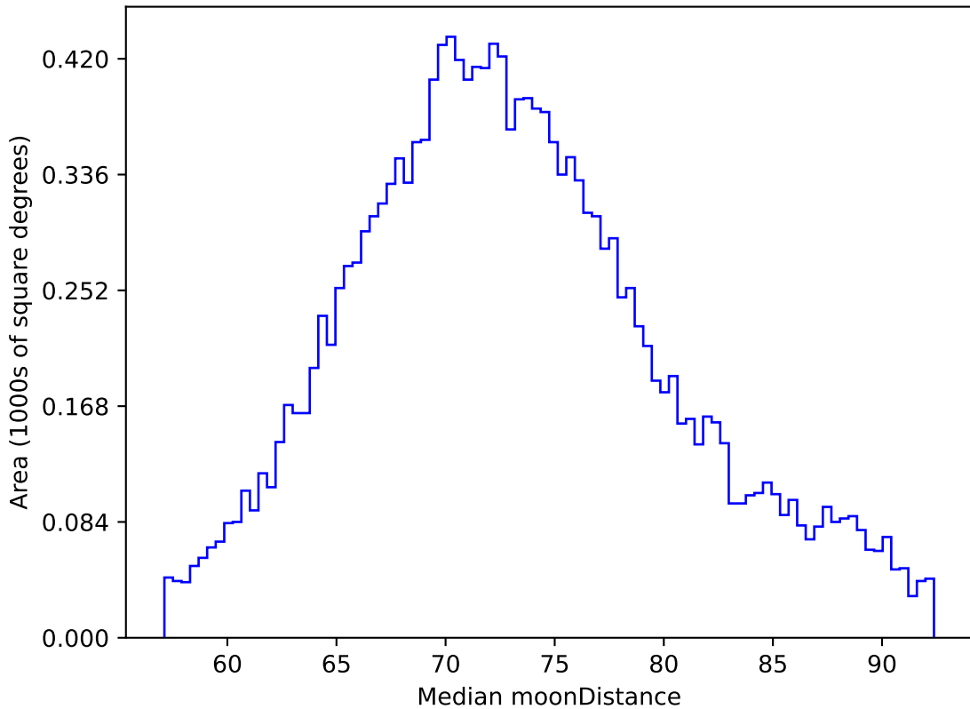
too_100_4v3.4_10yrs WFD z band: Median moonDistance
