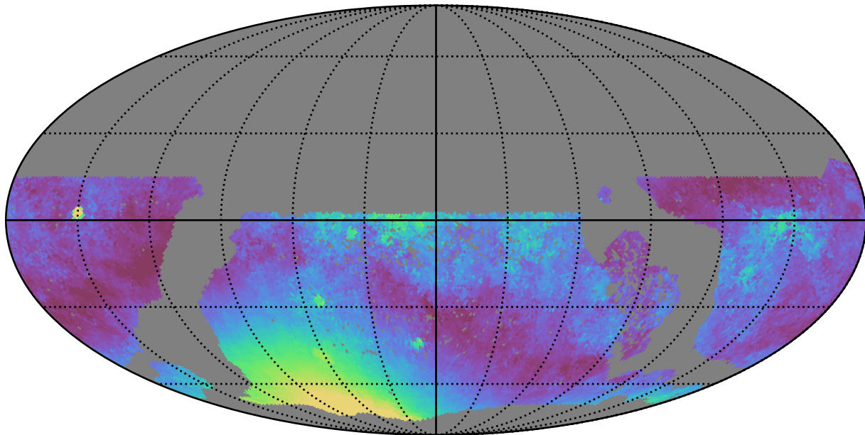
too_100_4v3.4_10yrs WFD y band: Median moonDistance
