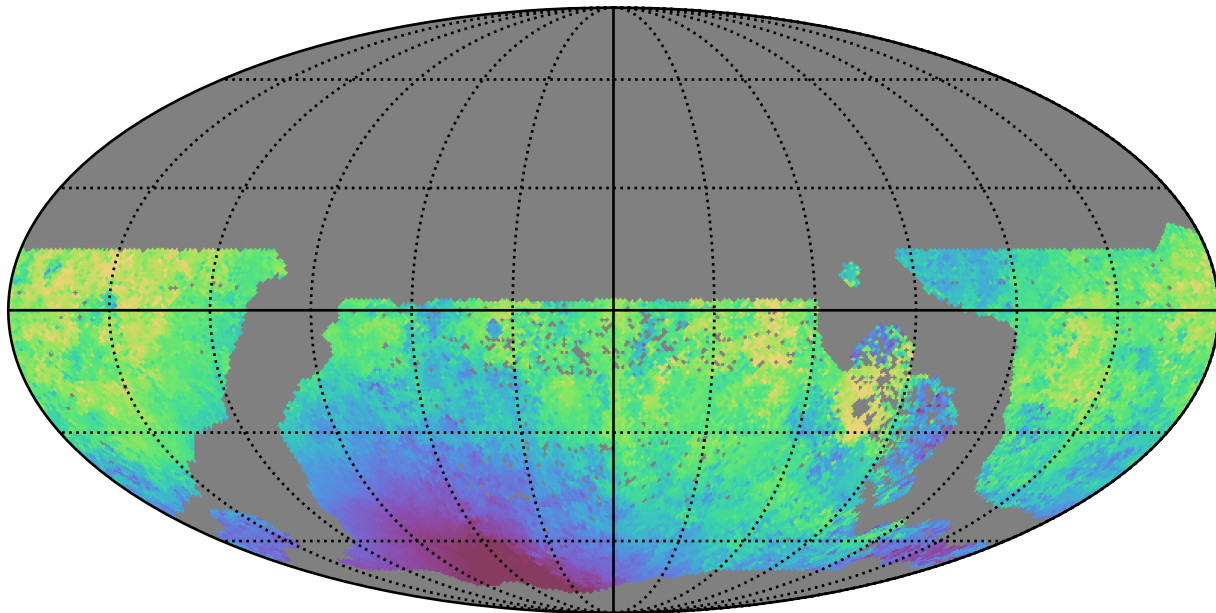
too_100_4v3.4_10yrs WFD u band: Median moonDistance
