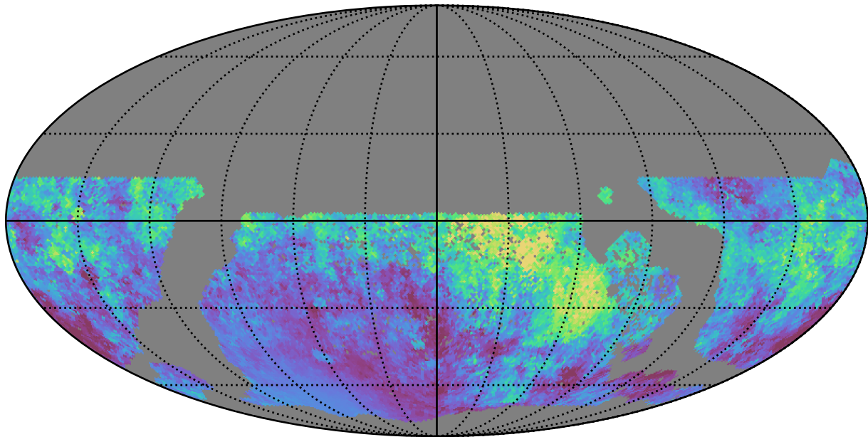
too_100_4v3.4_10yrs WFD i band: Median moonDistance
