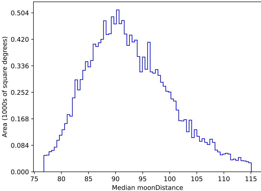
too_100_4v3.4_10yrs WFD i band: Median moonDistance
