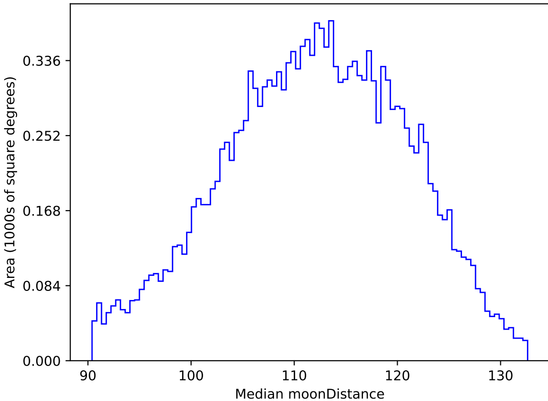
too_100_4v3.4_10yrs WFD g band: Median moonDistance
