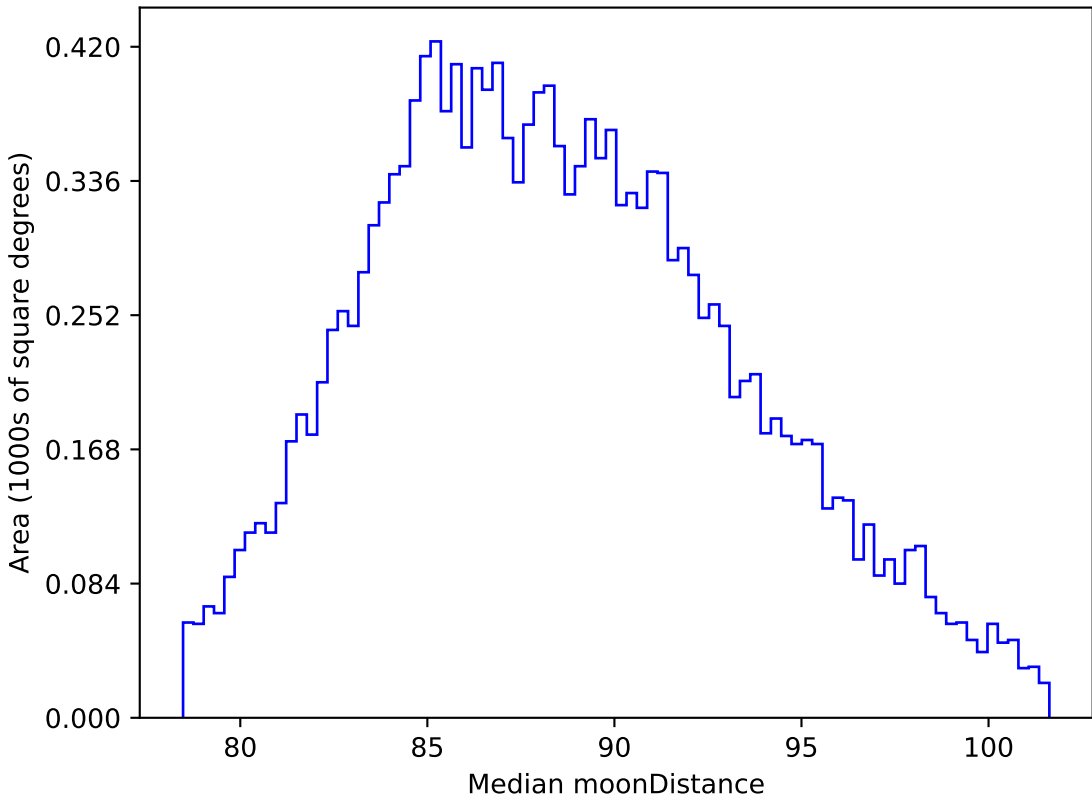
too_100_4v3.4_10yrs WFD all bands: Median moonDistance
