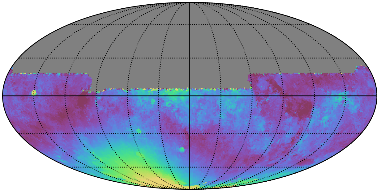
too_100_4v3.4_10yrs All sky y band: Median moonDistance
