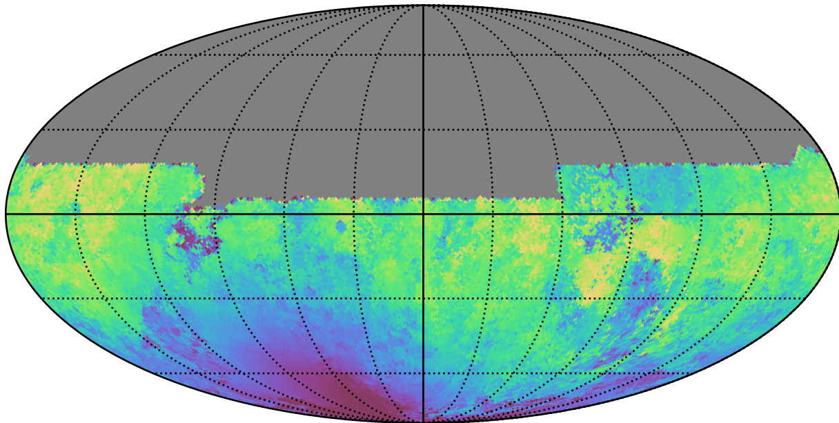
too_100_4v3.4_10yrs All sky u band: Median moonDistance
