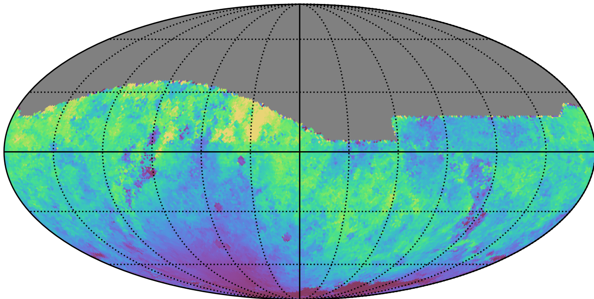
too_100_4v3.4_10yrs All sky r band: Median moonDistance
