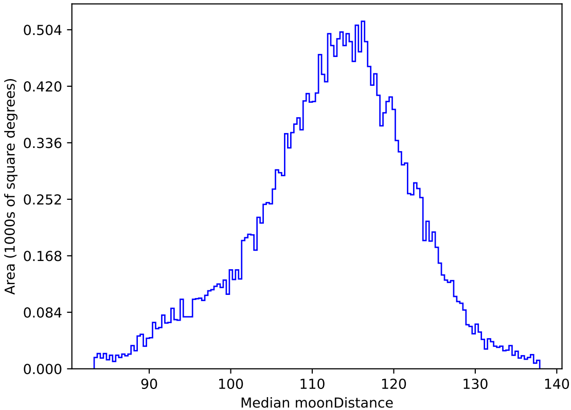
too_100_4v3.4_10yrs All sky r band: Median moonDistance
