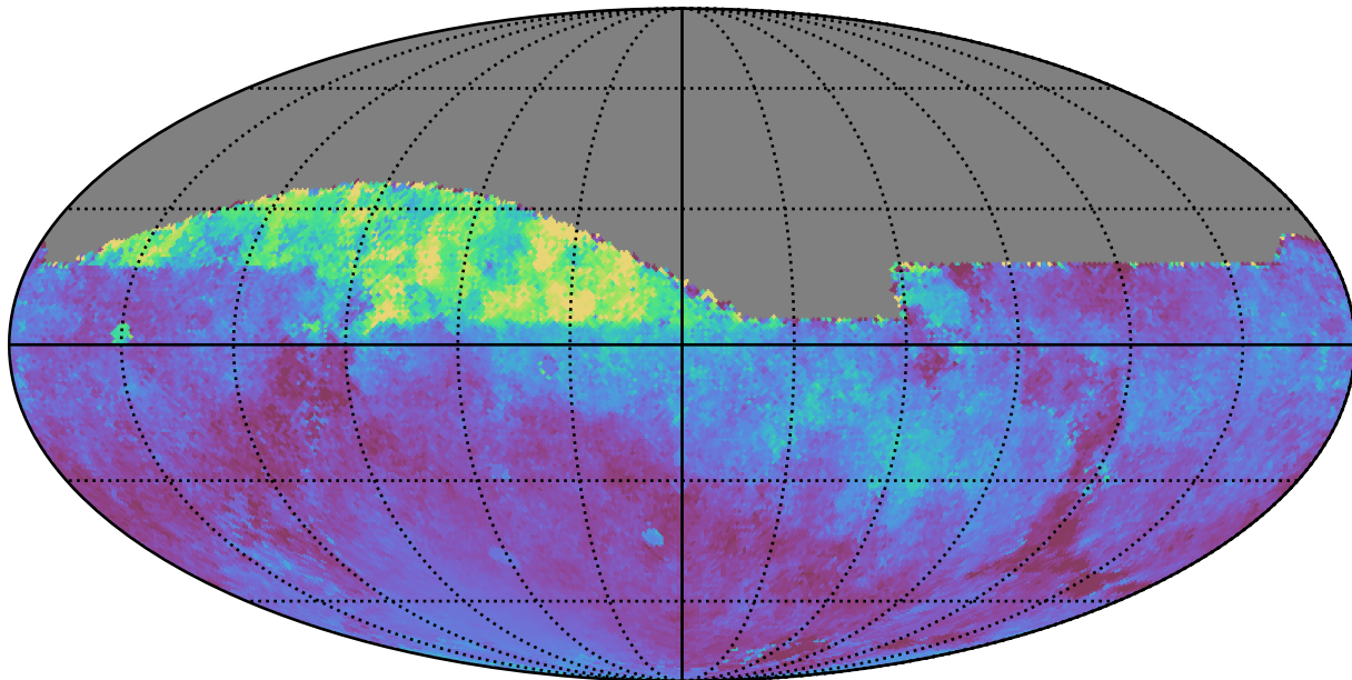
too_100_4v3.4_10yrs All sky all bands: Median moonDistance
