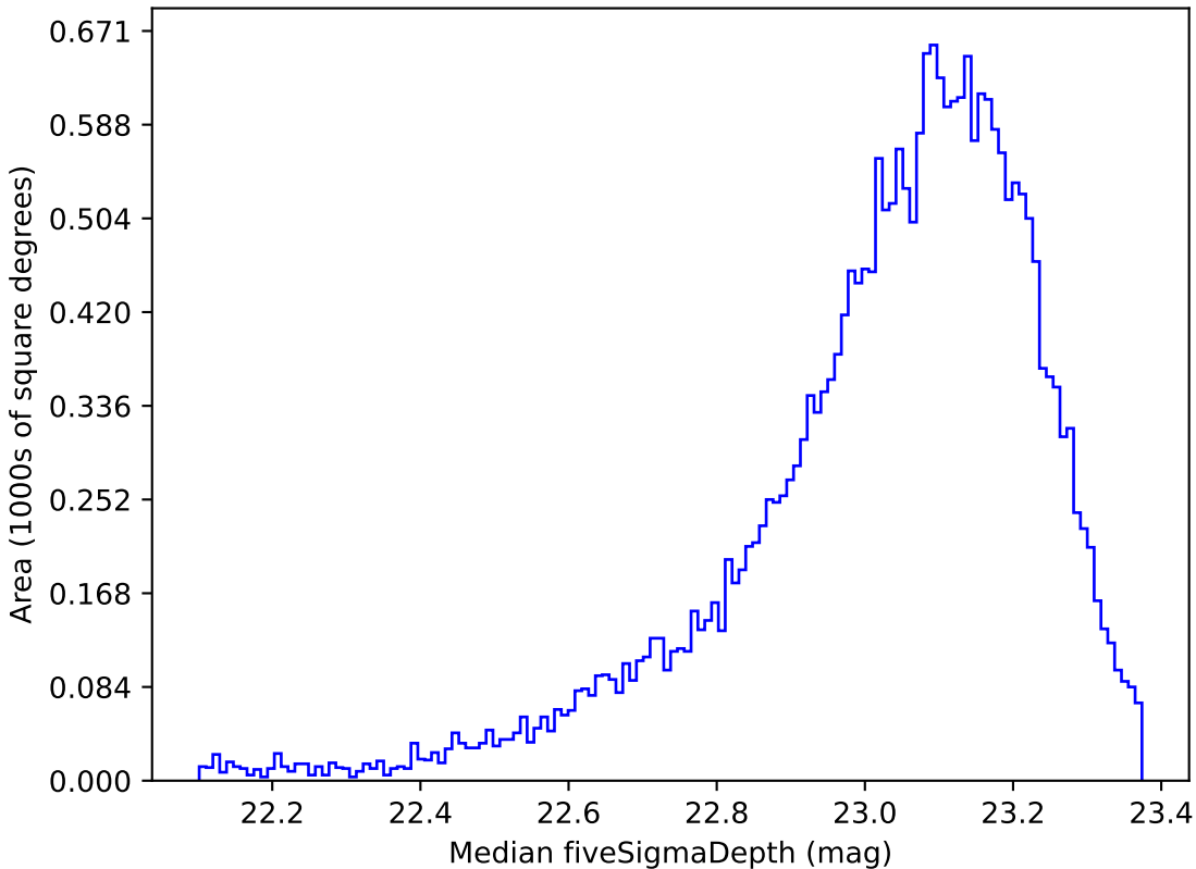
too_100_4v3.4_10yrs Yr 1 z band: Median fiveSigmaDepth
