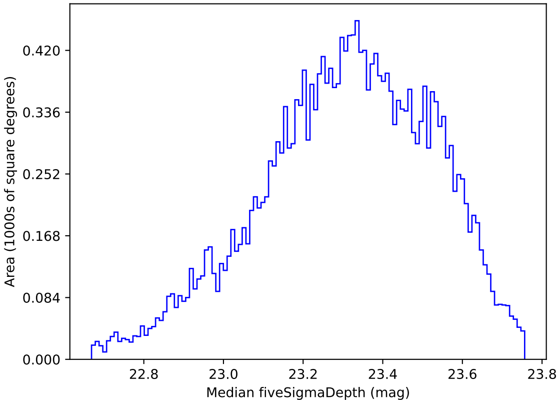
too_100_4v3.4_10yrs Yr 1 u band: Median fiveSigmaDepth
