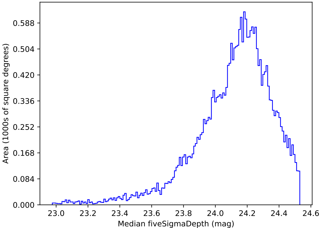
too_100_4v3.4_10yrs Yr 1 r band: Median fiveSigmaDepth
