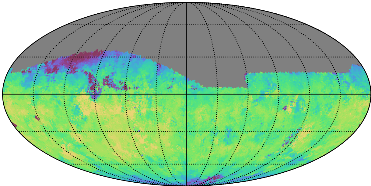
too_100_4v3.4_10yrs Yr 1 i band: Median fiveSigmaDepth
