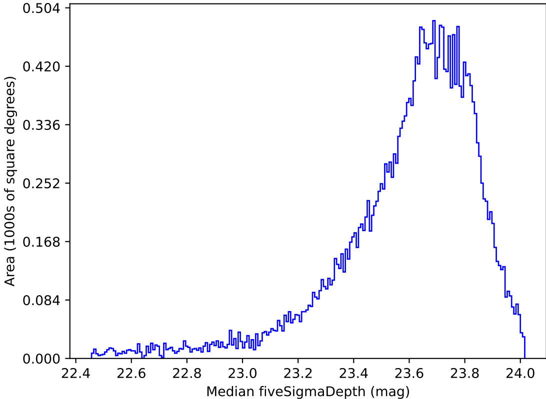
too_100_4v3.4_10yrs Yr 1 i band: Median fiveSigmaDepth
