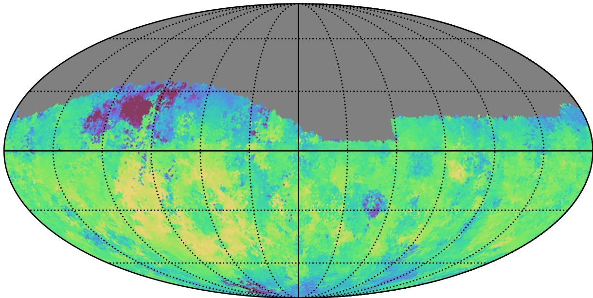
too_100_4v3.4_10yrs Yr 1 g band: Median fiveSigmaDepth
