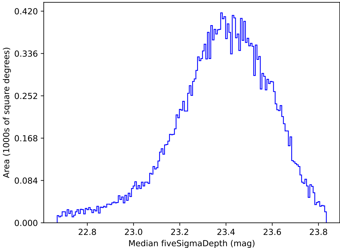
too_100_4v3.4_10yrs Yr 1 all bands: Median fiveSigmaDepth
