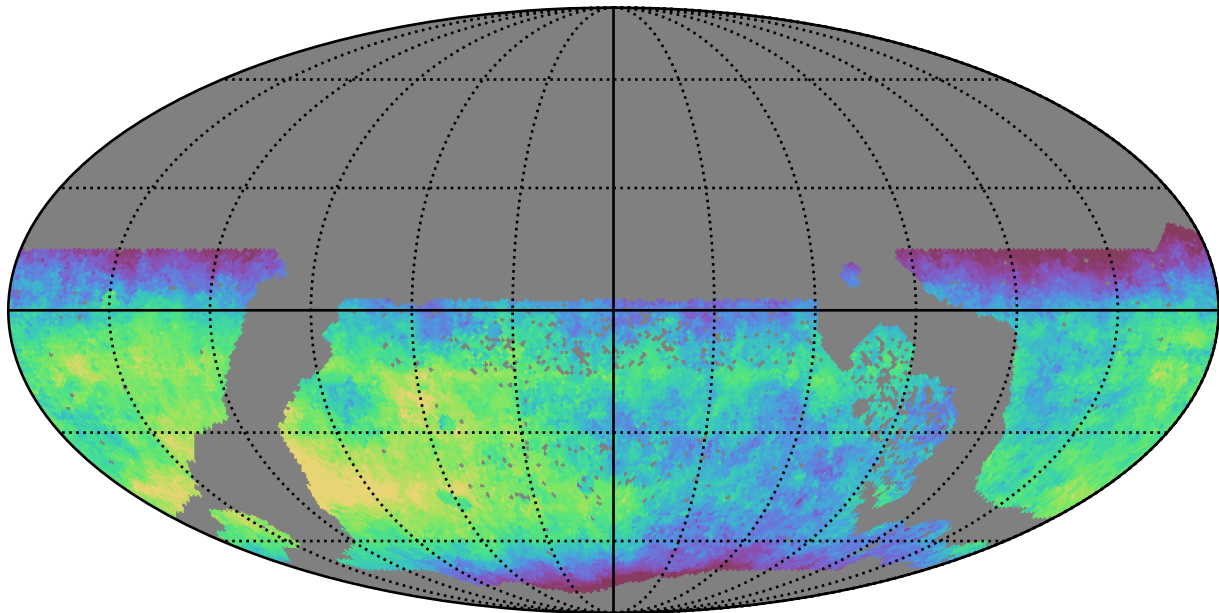
too_100_4v3.4_10yrs WFD z band: Median fiveSigmaDepth
