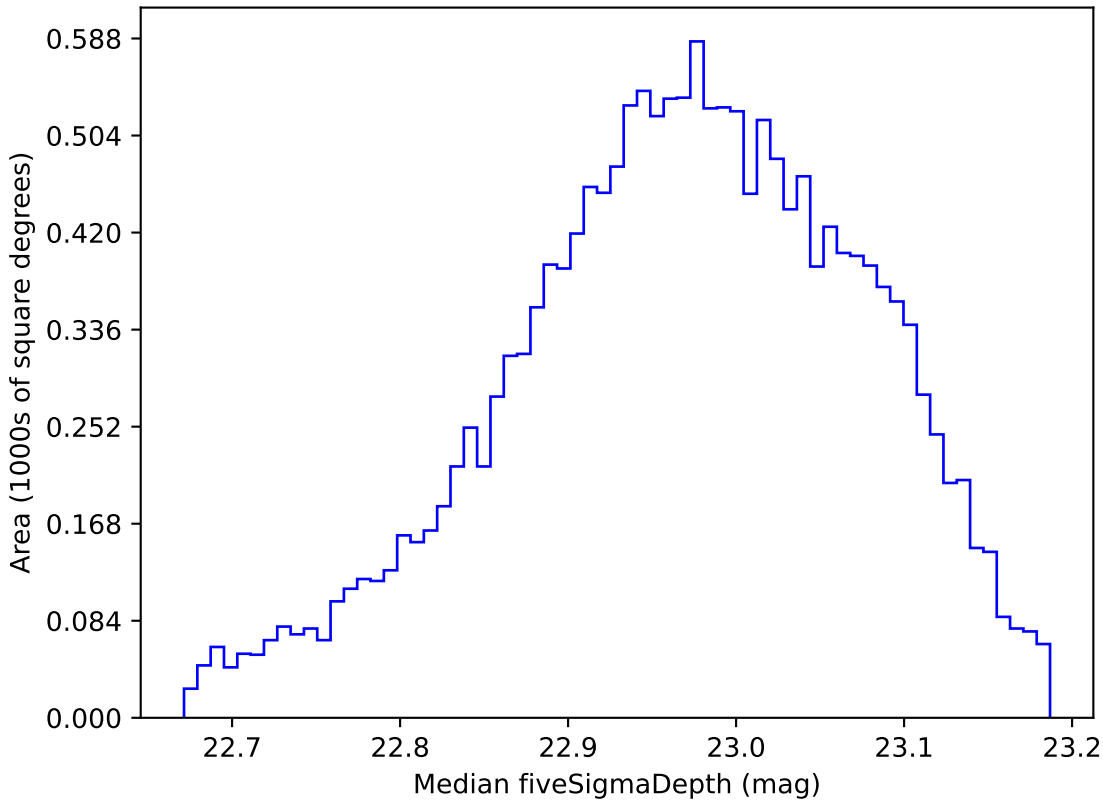
too_100_4v3.4_10yrs WFD z band: Median fiveSigmaDepth
