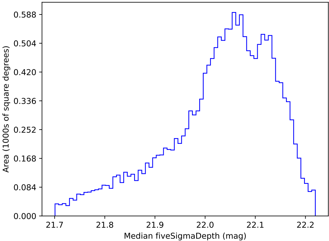
too_100_4v3.4_10yrs WFD y band: Median fiveSigmaDepth
