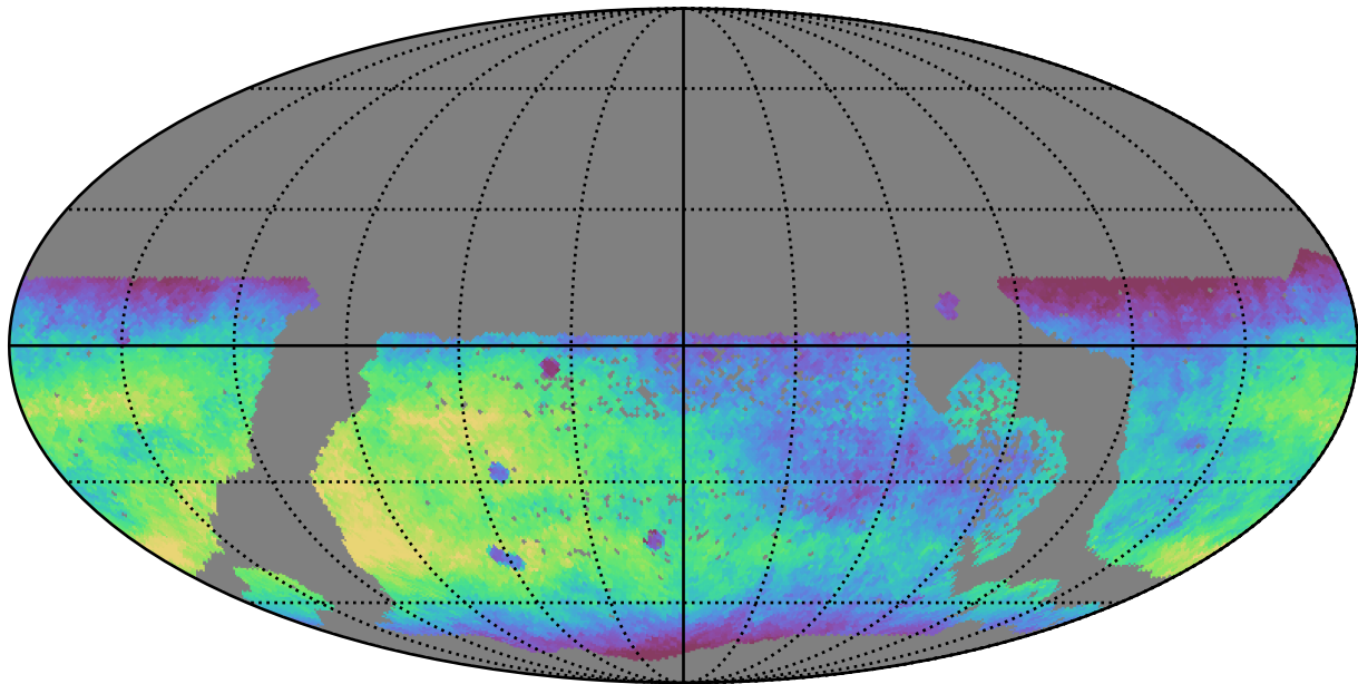
too_100_4v3.4_10yrs WFD r band: Median fiveSigmaDepth
