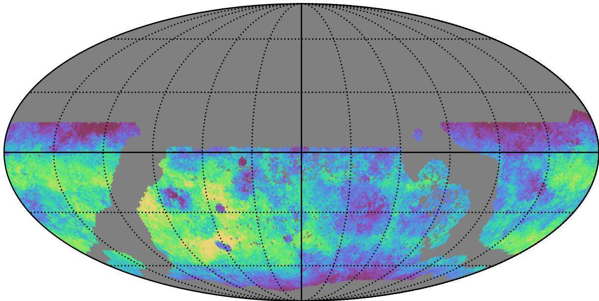
too_100_4v3.4_10yrs WFD g band: Median fiveSigmaDepth
